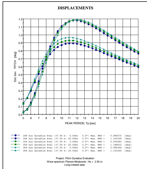
Figure 7: RMS Pitch vs. Peak Period
