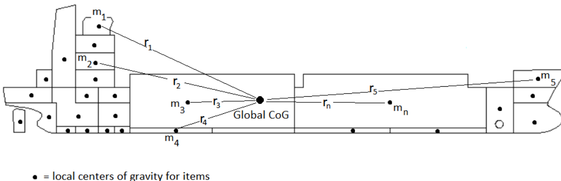
Figure 15: Parallel axis theorem applied on a vessel
