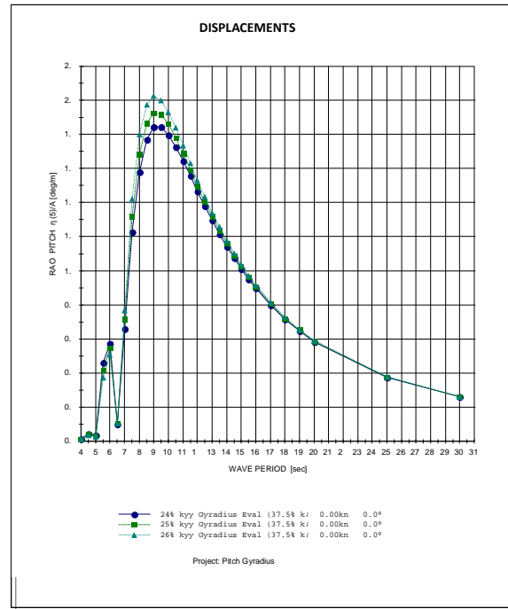
Figure 5: Pitch RAO vs. Wave Period
