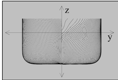
Figure 3: Series 60 Hullform Bodyplan
