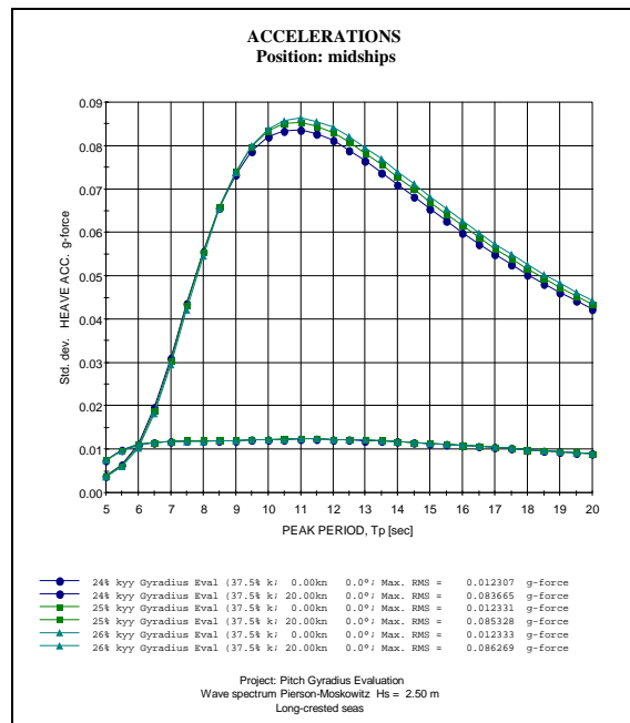
Figure 9: RMS Heave Acceleration @ Midships vs. Peak Period
