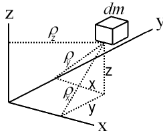
Figure 1: Calculating inertia of an object by integration
