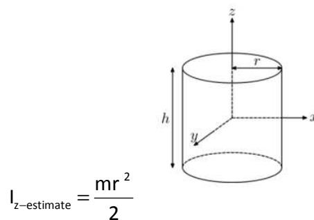
Figure 13: MOI of a solid cylinder
